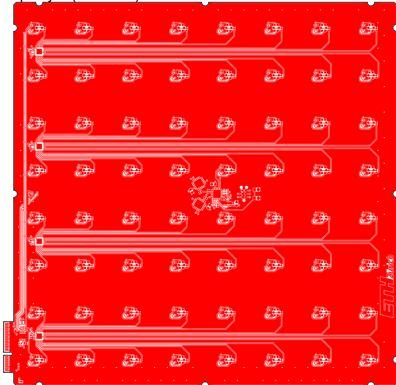
Int1 (Signal) (Scale 2:3)
