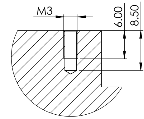
DETAIL G SCALE 2 : 1
