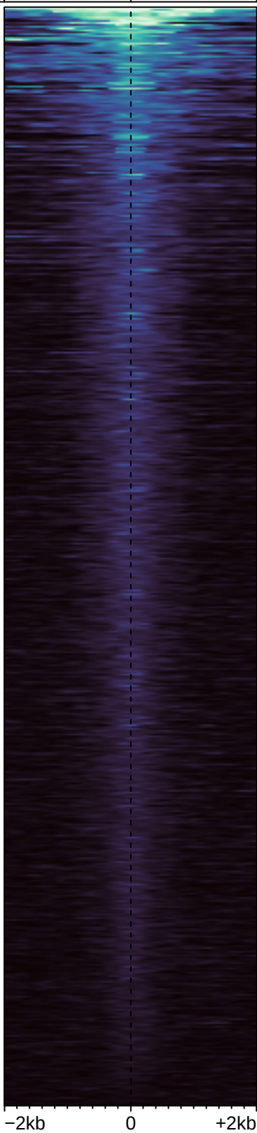
GR-ChIP sites
