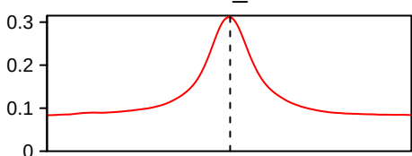
fused_uds
