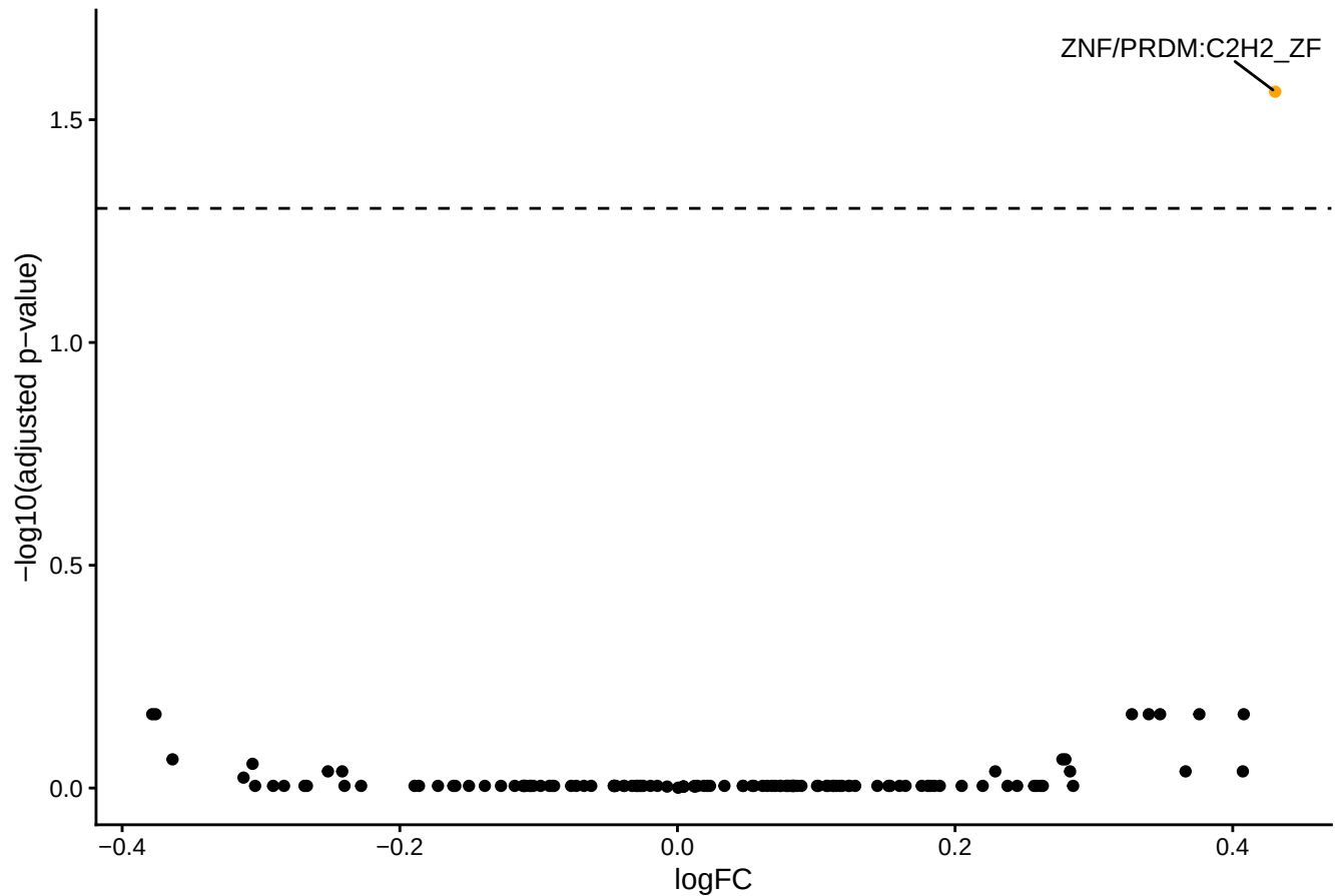
MotifActivity (Archetype) of H3K4me3 embryonal signal in Stress vs Ctrl
