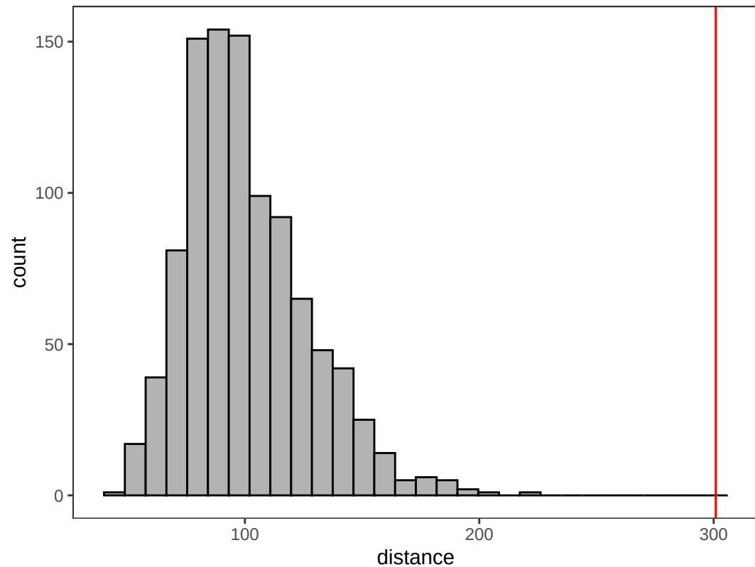
Control-vs-IFS kmeans.50
