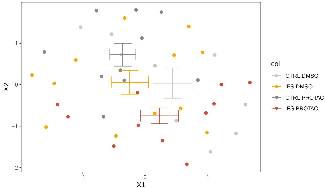
Syllable Count CTRL-vs-IFS offspring males
