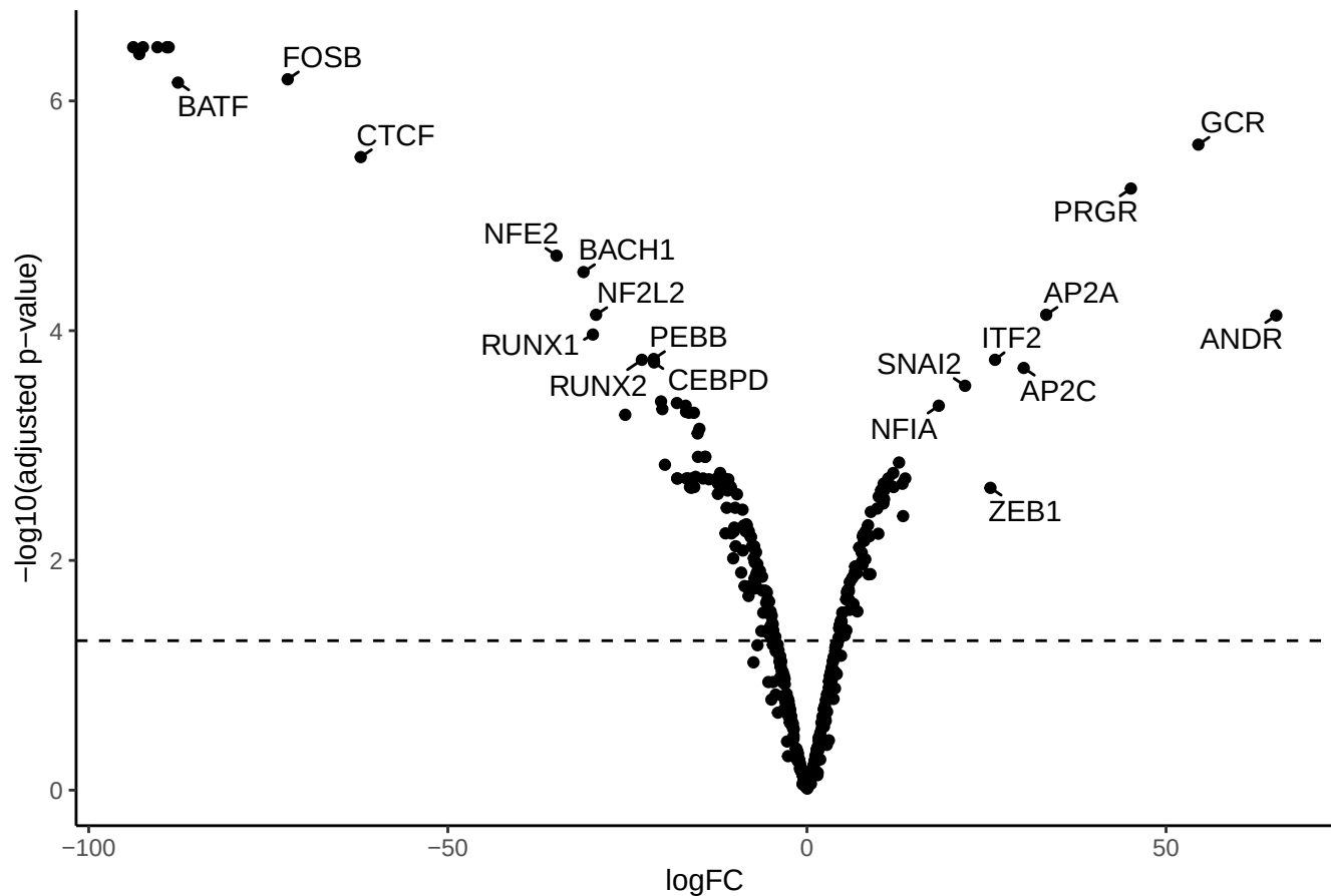
Transcription factor motif activity spermatozoa vs MIIoocyte
