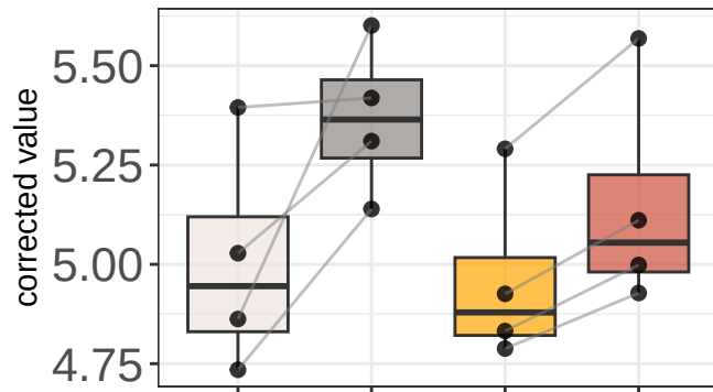
tRNA_Leu_AAG_3_end top3 in KH-103 vs DMSO
