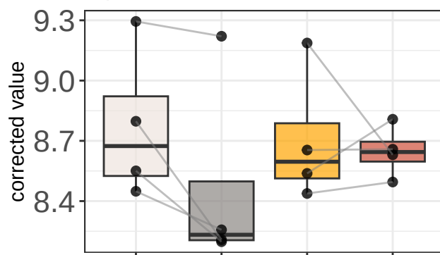
tRNA_Leu_CAG_5_end top2 in KH-103 vs DMSO
