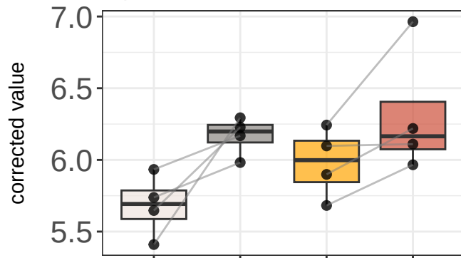
tRNA_Gly_GCC_3_end top1 in KH-103 vs DMSO
