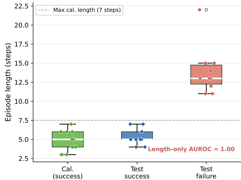
Push-Chair: Failure ↔ Duration
