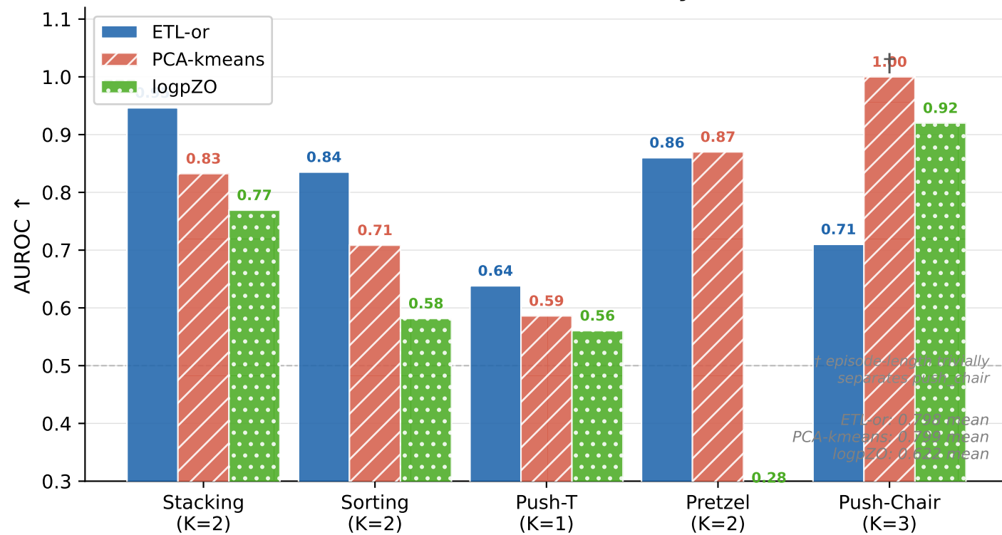
Failure Detection AUROC by Task
