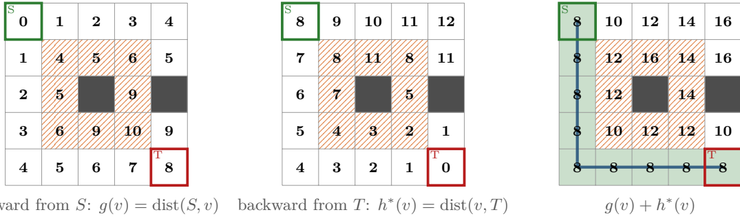
Figure 3.6. Forward and backward tables on the grid of Example 3.5, both from full runs. Left: g(v) = \text{dist}(S, v) from S . Middle: h^*(v) = \text{dist}(v, T) from Algorithm 3.2; because entering a slow cell costs 3 but leaving it costs 1, this is not the distance from T (compare h^*(3, 3) = 2 with the 4 that a forward run from T gives). Right: g(v) + h^*(v) , the cost of the best path from S to T through v . The green cells, where the sum equals \text{dist}(S, T) = 8 , are exactly the cells of the optimal path; every other cell has a larger sum, which is how A^* will know to avoid them.
