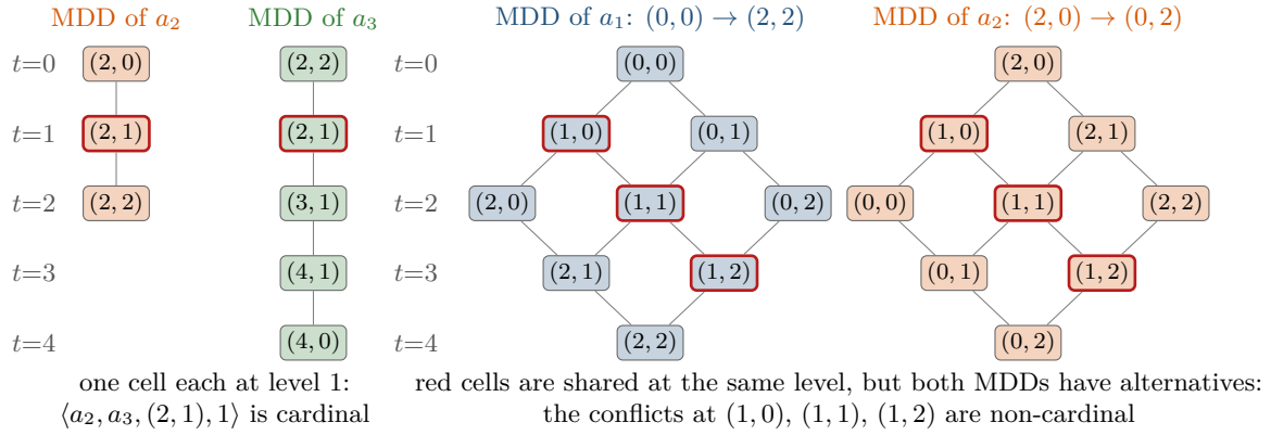
Figure 9.4. Multi-valued decision diagrams. Left: at the root of Example 9.4 the MDDs of a_2 and a_3 are chains that share the cell (2, 1) at level 1, so the conflict there is cardinal. Right: in an open 3 \times 3 room the MDDs of two crossing agents are wide; the shared cells (red) have alternatives on both sides, so every conflict is non-cardinal and a split does not raise the cost.
