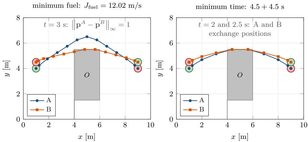
Figure 22.4. Optimal trajectories of Example 22.6, sampled every \Delta t = 0.5 s (dots), for the minimum-fuel objective (left) and the minimum-time objective (right); the gray rectangle is the inflated block. Left: A (blue) climbs over B (orange) and the two pass at t = 3 s with exactly d_{\min} = 1 m of \infty -norm separation. Right: both drones arrive after 4.5 s at full acceleration, hug the top edge of the block, and swap their x -positions between t = 2 and t = 2.5 s: every sampled separation is at least 1.25 m, yet the continuous paths cross. The constraints hold only where they are imposed.
