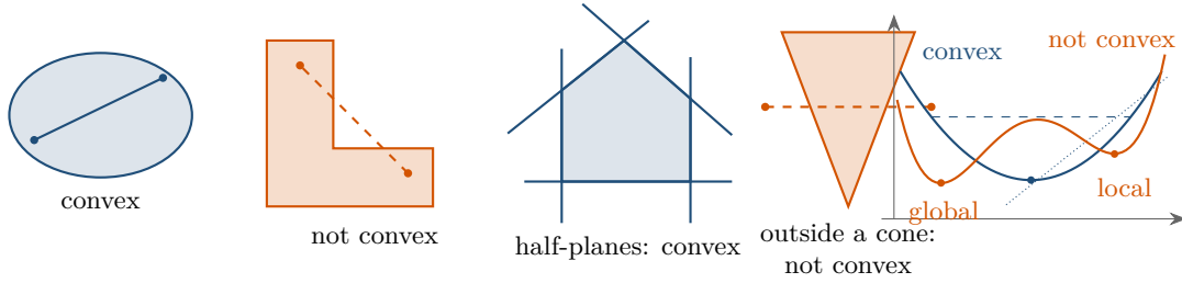
Figure B.2. Convexity. Left: in a convex set every chord stays inside; in the non-convex set the dashed chord leaves it. Middle: an intersection of half-planes, the situation of ORCA in Chapter 13, is convex, while the set of velocities outside a cone, the situation of a velocity obstacle in Chapter 12, is not. Right: a convex function lies below its chords and above its tangents, so its only stationary point is the global minimum; the non-convex function has a local minimum in which gradient descent can stop.
