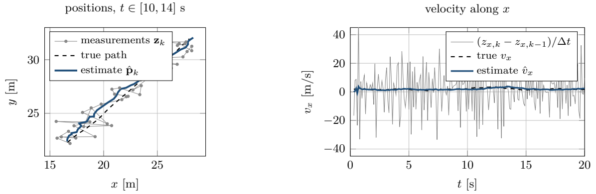
Figure 18.1. Why raw measurements are unusable for planning. Left: four seconds of the experiment of Section 18.9 , position reports at 10 Hz with noise 1 m along x and 0.5 m along y (gray), the true path (dashed) and the Kalman estimate (blue). Right: the velocity v_x from differencing consecutive reports (gray) swings by tens of meters per second, while the filter’s estimate (blue) follows the true velocity (dashed) to within a fraction of a meter per second.
