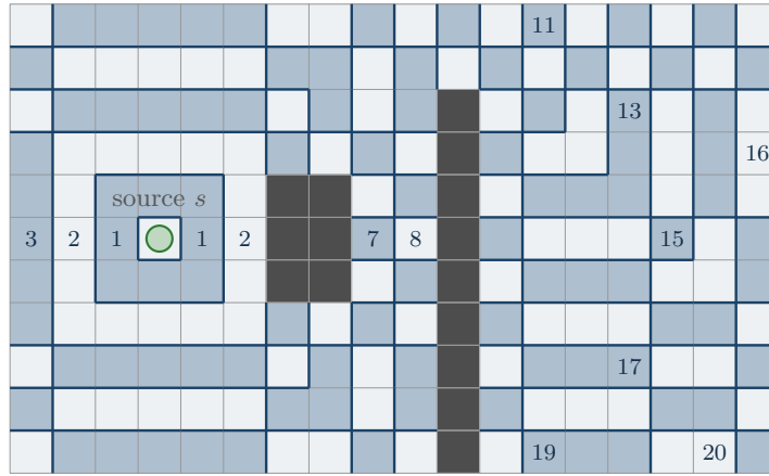
Figure 3.1. Dijkstra's algorithm as a spreading wave on an 8-connected grid (diagonal moves cost \sqrt{2} ). Cells are shaded by the band \lfloor g \rfloor of their cost from the source; the wave settles every cell of band k before any cell of band k + 1 , bends around the block and passes through the gap at the top of the wall. Behind the wall the bands are centered on the gap, not on the source: cost is measured along paths, not as the crow flies.
