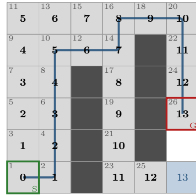
(b) Dijkstra ( h = 0 ): 26 expansions
