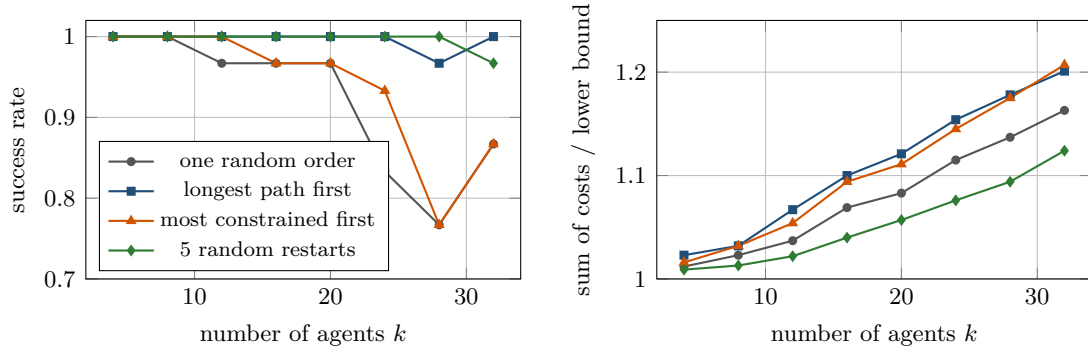
Figure 8.6. Priority ordering rules on random 20 \times 20 grids with 20% obstacles (thirty instances per k , HCA*). Left: fraction of instances solved. Right: sum of costs relative to the sum of the independent shortest paths, over the instances solved by all four rules. Longest path first almost never fails; it and most constrained first produce the most expensive plans (within one point of each other for k \geq 24 ); five random restarts give the cheapest plans and fail once in 240 instances.
