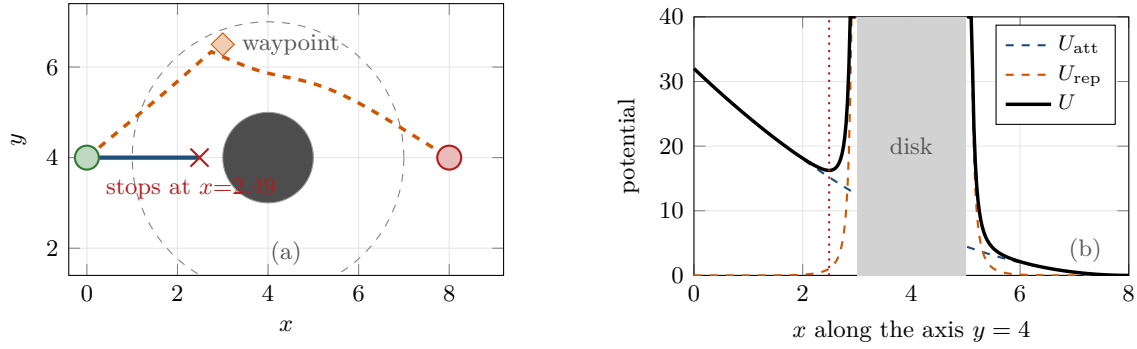
Figure 15.4. Failure mode 1: local minimum. (a) From (0, 4) the drone stops at x = 2.49 , where the attraction ( 8 - x ) and the repulsion cancel; the dashed orange path is the same drone steered through a waypoint at (3, 6.5) from a global planner (Section 15.8). (b) The potentials along the axis y = 4 : attractive bowl (blue), repulsive chimney (orange) and their sum (black), with a dip at x = 2.49 (dotted red line).
