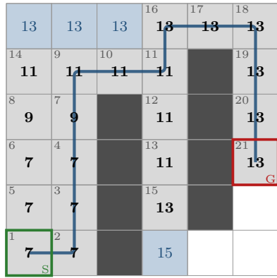
(a) A*, Manhattan h : 21 expansions
