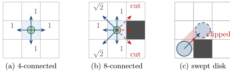
Figure 2.1. Grid connectivity. (a) The four straight moves of G_4 cost 1 each. (b) In G_8 the diagonal moves cost \sqrt{2} ; the move into the obstacle is forbidden because the cell is blocked, and the two diagonals past its corners are forbidden by the corner-cutting rule. (c) Why: a disk that slides diagonally past an obstacle corner clips it, even though the start and end cells are free.
