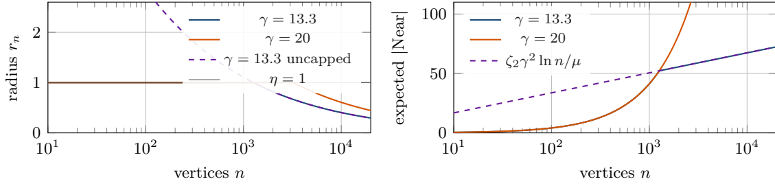
Figure 17.2. Left: the connection radius of Equation (17.1) for the map of Example 17.7 ( \mu = 76 , d = 2 , \eta = 1 ) with the chapter’s \gamma = 13.3 (blue) and with \gamma = 20 (orange). The cap \eta is active while the tree is small, and for longer with the larger constant; the dashed curve is the uncapped schedule for \gamma = 13.3 . Right: the expected size of the NEAR set, n\zeta_2 r_n^2 / \mu , for the same two constants. It grows linearly while the cap is active and then follows \zeta_2 \gamma^2 \ln n / \mu (dashed, \gamma = 13.3 ): the \gamma = 20 curve sits a factor (20/13.3)^2 = 2.3 above it, which is what more rewiring per iteration costs.
