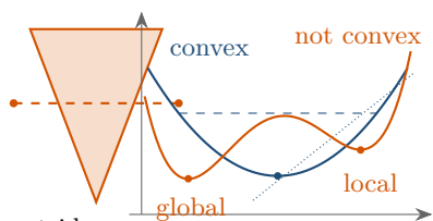
outside a cone: not convex
