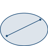
convex
