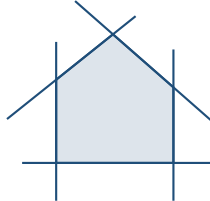
half-planes: convex
