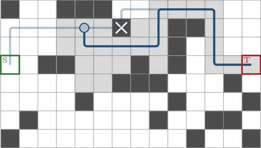
A^* from scratch: 26 expansions
