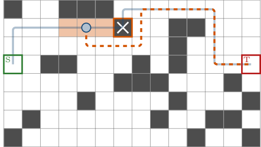
D^* Lite repair: 6 expansions
