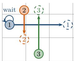
(b) plan Y: agent 1 wait SoC = 10, MS = 5
