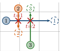
(a) shortest paths: two vertex conflicts
