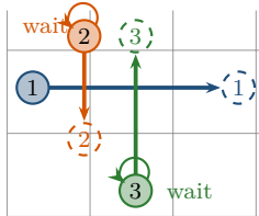
plan X: agents 2 and 3 wait once SoC = 11, MS = 4
