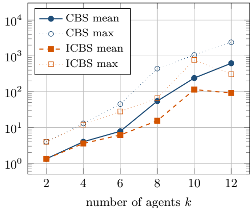
CT nodes expanded (solved runs)
