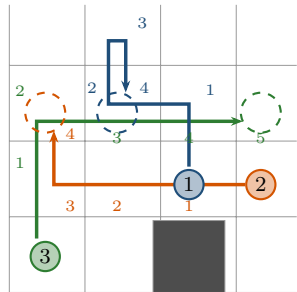
(c) ECBS (1.2): cost 13, a_1 steps aside to (0,1)
