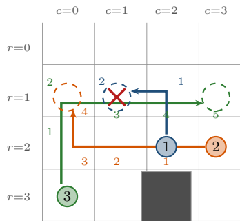
(a) root: cost 11, a_1 and a_3 at (1,1) , t=3
