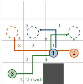
(b) CBS: cost 12, a_3 waits once at (3,1)
