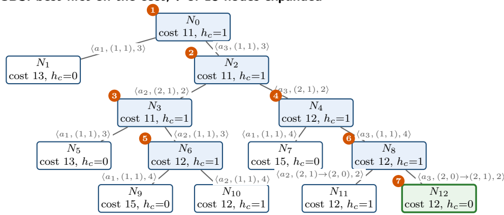
(a) CBS: best-first on the cost; 7 of 13 nodes expanded
