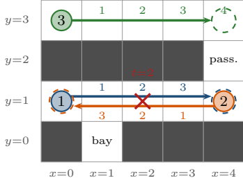
(a) individual policies: agents 1 and 2 collide in cell (2, 1) at t = 2 (b) plan of cost 15: agent 1 waits at (1, 1), hides in the bay while agent 2 passes, and continues
