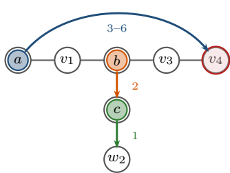
(a) push: a walks to v_4 ; the blockers b and c shift one step down the branch
