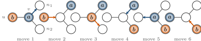
(b) swap: at a vertex v of degree \geq 3 with two empty neighbors n_1, n_2 , six moves exchange a and b without moving anyone else
