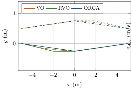
trajectories (A solid, B dashed)
