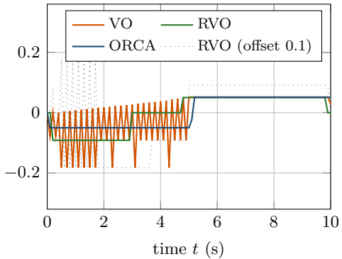
lateral velocity of A
