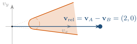
(b) \mathbf{v}_{\text{rel}} lies inside VO_{A|B}^{\tau} : collision before
