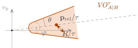
(a) truncated VO, apex \mathbf{0} , legs tangent to the
