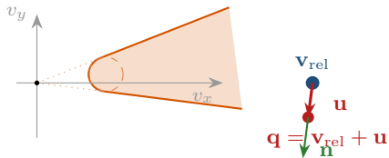
shortest way to the boundary (right leg); \mathbf{n} : out
