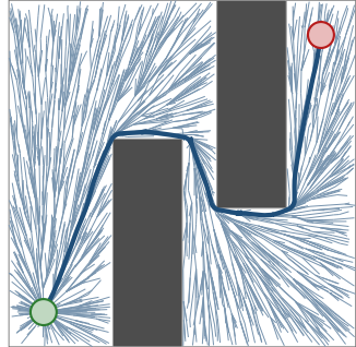
(c) 3000 iterations 2193 vertices, cost 17.32
