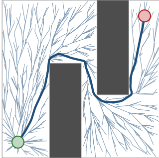
(b) 1000 iterations 680 vertices, cost 18.21
