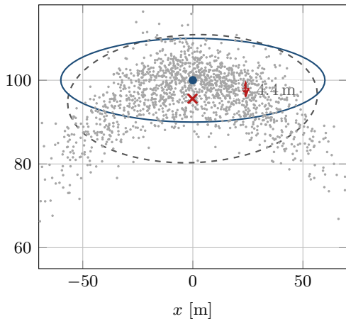
(a) EKF: the tangent at the mean
