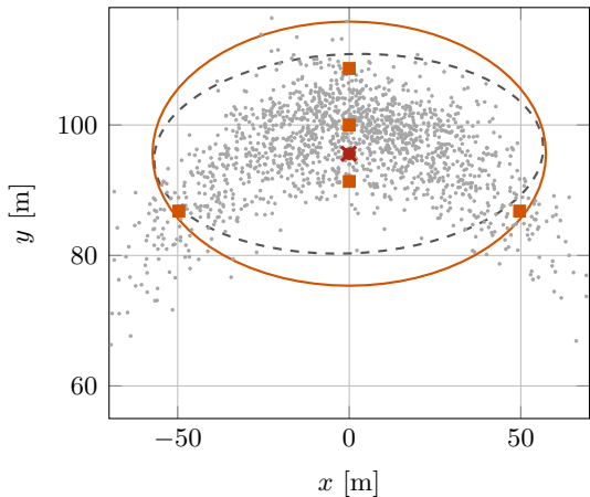
(b) UKF: five sigma points
