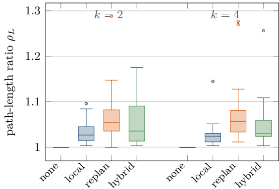
path length relative to the nominal plan
