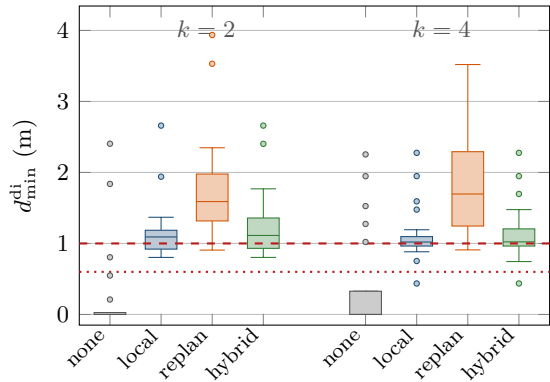
minimum drone-intruder separation
