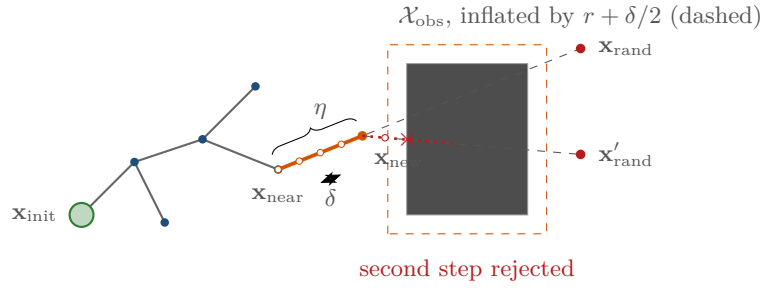
Figure 16.2. The primitives of one iteration. The sample \mathbf{x}_{\text{rand}} selects the nearest vertex \mathbf{x}_{\text{near}} ; STEER moves at most \eta toward the sample and proposes \mathbf{x}_{\text{new}} ; COLLISIONFREE tests points spaced \delta apart along the new segment against the obstacle inflated by r + \delta/2 (dashed), which is conservative by Proposition 16.3. The second attempt, from \mathbf{x}_{\text{new}} toward \mathbf{x}'_{\text{rand}} , is rejected because its second test point falls inside the inflated region; no vertex is added.
