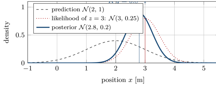
Figure 18.3. The one-dimensional update of Example 18.6. The prediction (gray, dashed) and the likelihood of the measurement (red, dotted) multiply to the posterior (blue), which is narrower than both and centered at \hat{x} = \hat{x}^- + Ky with K = 0.8 . The wider density contributes less to the position of the peak: the arrow is 80% of the way from \hat{x}^- to z .
