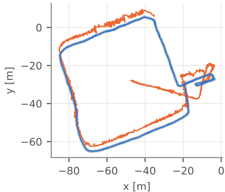
Oxford Spires keble-college-03 (Hesai QT64) APE: KISS-SLAM 9.76 m · ours 0.09 m
