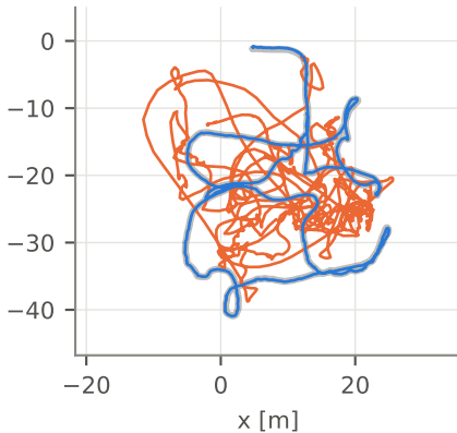
Newer College underground_hard (Ouster 128) APE: KISS-SLAM 12.78 m · ours 0.09 m
