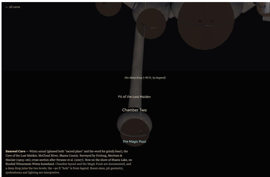
Figure 10: Samwel Cave, the descent: Chamber One, the deep drop (the ~90 ft “hole” of legend), and Chamber Two with the glowing Magic Pool at the bottom. The on-screen caption marks documented vs. interpretive features and the contested gloss of sawal .
