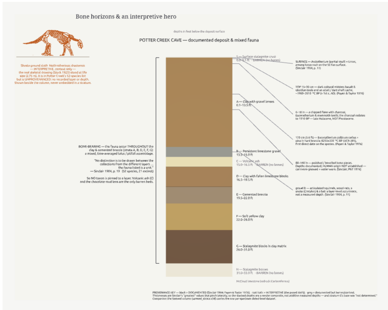
Figure 8: Potter Creek bone-horizon section (interpretive hero at left, documented column at centre, cited depth-callouts at right). Sinclair's strata are drawn to scale; fauna are pinned only at documented depths (the 170 cm Euceratherium date; the depth-documented but human-origin-refuted polished bone). The mixed assemblage is a single bracketed marker quoting Sinclair's "the fauna listed is a unit" (p. 19); the ground-sloth skeleton (Stock 1925) is flagged interpretive and unprovenanced, standing beside — never inside — the deposit. Thicknesses are Sinclair's "greatest" values, so the stacked depths are a render composite, which the legend states.
