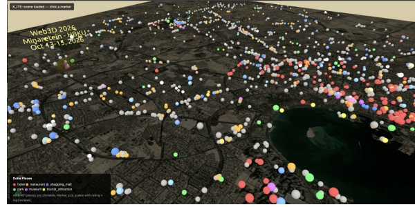
Figure 3: The Doha, Qatar scene rendered in X_ITE. Terrain comes from the Google Elevation API, place markers (restaurants, hotels, museums, tourist attractions, shopping malls, parks) from the Google Places API, and each marker is clickable to surface its rating. The X3D scene graph is fully validated against the X3D 4.0 XSD.
