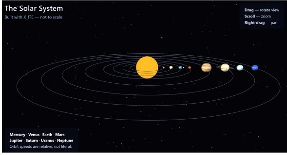
Figure 2: The Solar System scene rendered in X_ITE after three iterative turns: compose_scene for geometry and placement, per-planet animate_x3d_node calls for TimeSensor/OrientationInterpolator/ROUTE chains, and modify_x3d_node for texturing. XSD- and semantically valid at every turn.
