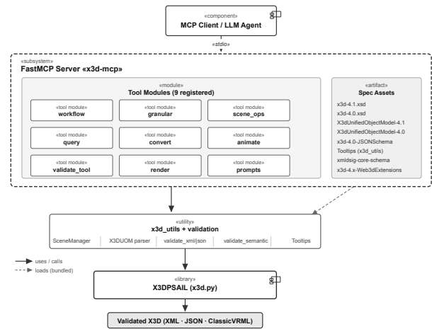
Figure 1: x3d_mcp architecture. The MCP client (e.g., Claude Desktop) invokes tools via JSON-RPC over stdio. The server dispatches each call into one of nine tool modules; scene construction is performed by X3DPSAIL, queries are answered from the in-memory X3DUOM index, and every artifact is validated against the bundled X3D 4.0/4.1 schemas before being returned.
