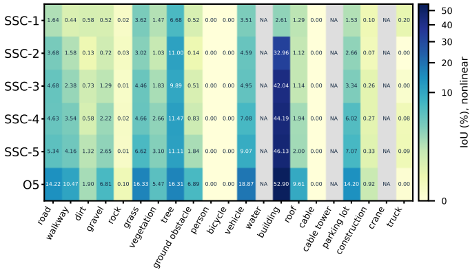
OccuFly test per-class IoU (%)
