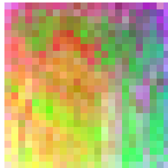
Predicted depth
