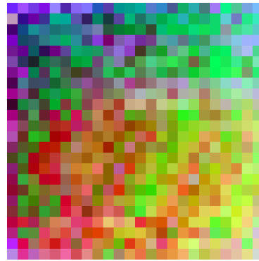
Tubelet - 0
