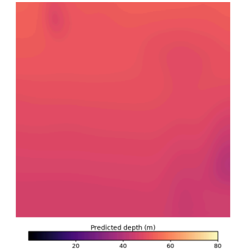
Predicted depth
