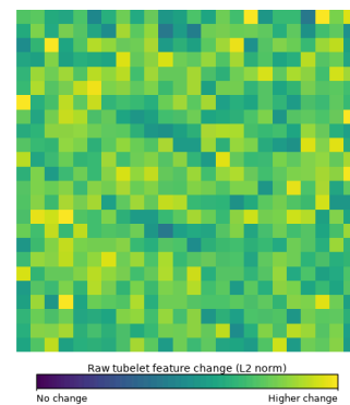
Tubelet 0 & 1 feature change
