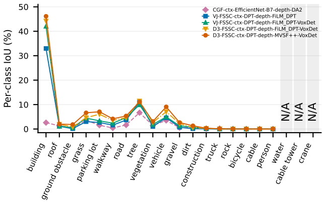
(b) Semantic completion
