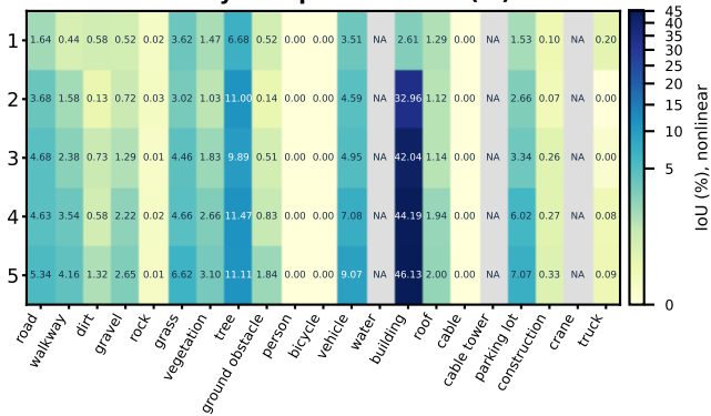
OccuFly test per-class IoU (%)
