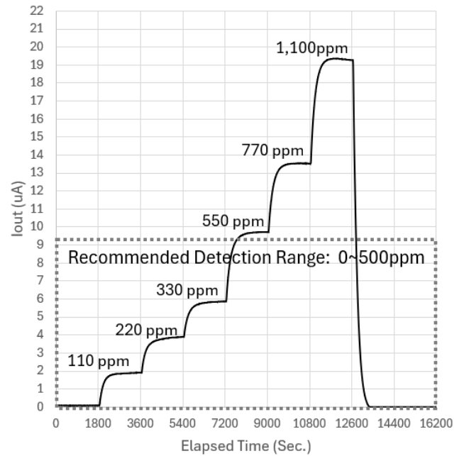
Figure 3 Recommended Detection Range
