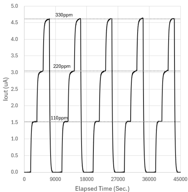
Figure 4 Repeatability
