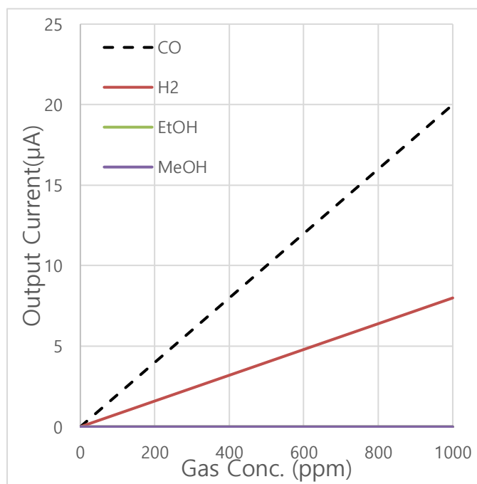
Figure 1 Interference gas sensitivity
