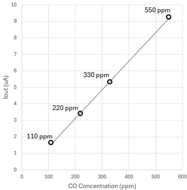
Figure 2 Linearity
