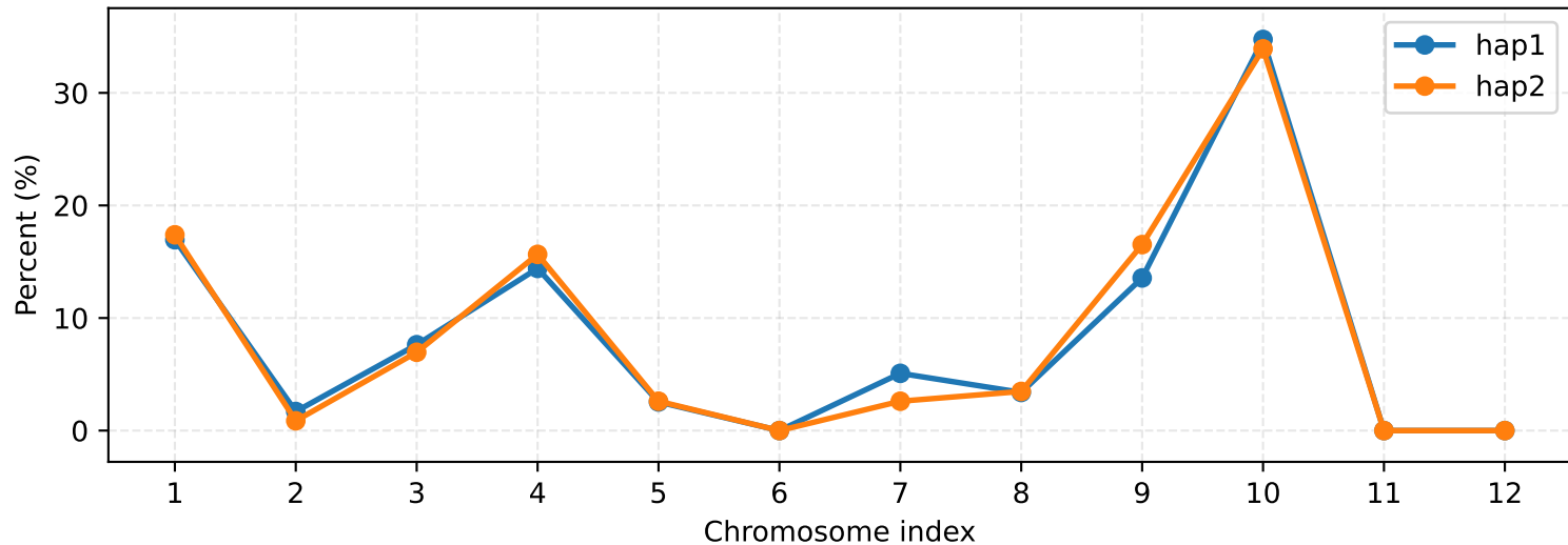
ACH — Chromosome share within family (% , by hap)
