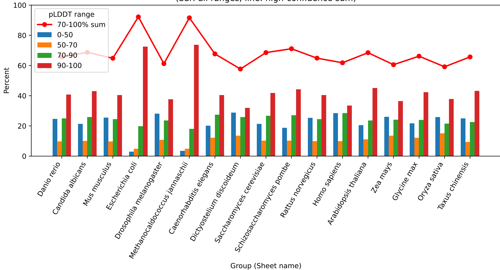
pLDDT Range Distribution per Group (bar: all ranges; line: high-confidence sum)
