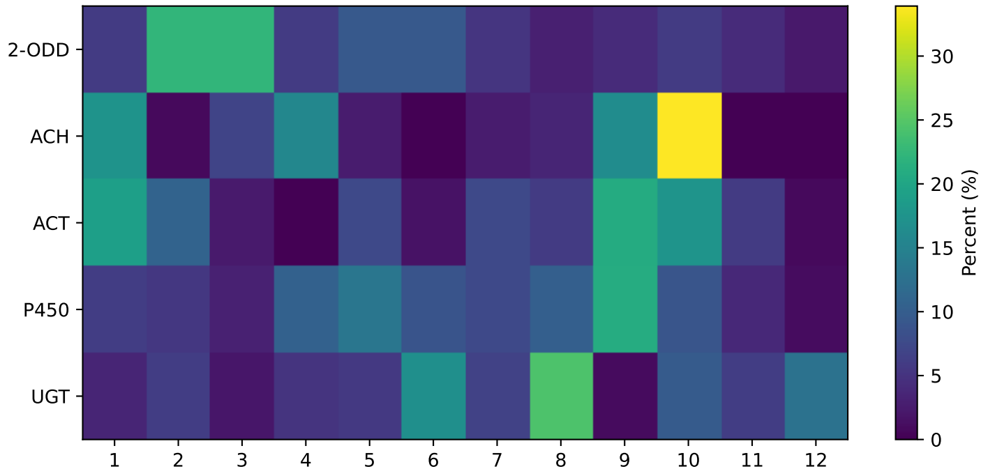
Chromosome share within family (% , hap2)
