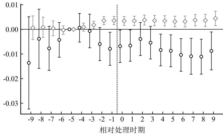
(a) TWFE
