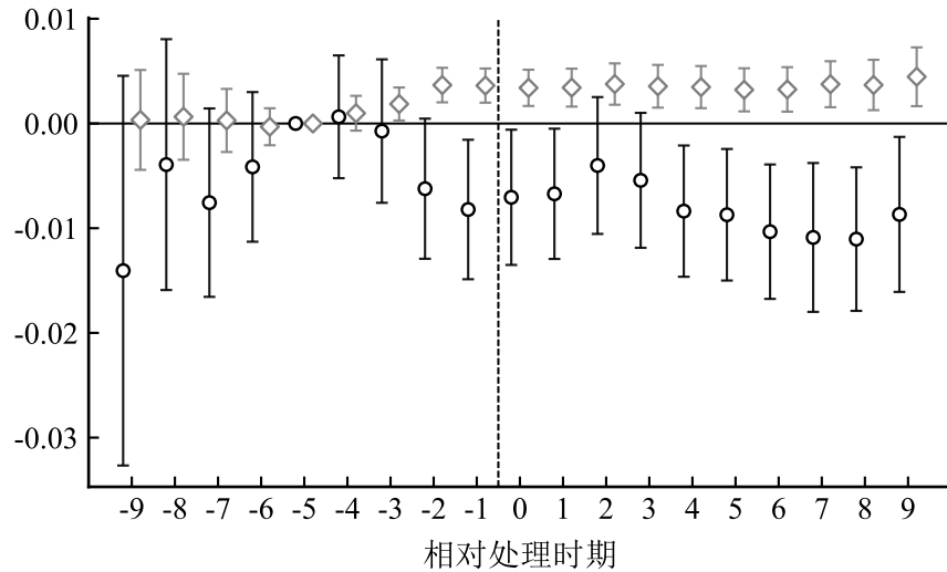
(b) Stacked
