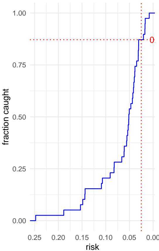
Full Model – Empirical CDF of
