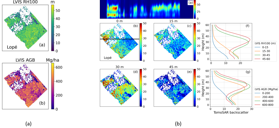
Figure 15: TomoSAR sensitivity to forest height and biomass. (a) Lidar reference data showing forest height (RH100, 0-50m) and AGB (0-600 Mg/ha) over Lopé, Gabon. (b) TomoSAR backscatter profiles for different height classes (0-15m, 15-30m, 30-45m, 45-60m) and AGB classes (0-200, 200-400, 400-600, 600-800 Mg/ha). Profiles systematically shift in height and shape with increasing forest height and biomass, demonstrating TomoSAR’s sensitivity to forest structure. AfriSAR airborne campaign data. Source: Liu et al. (2024)
