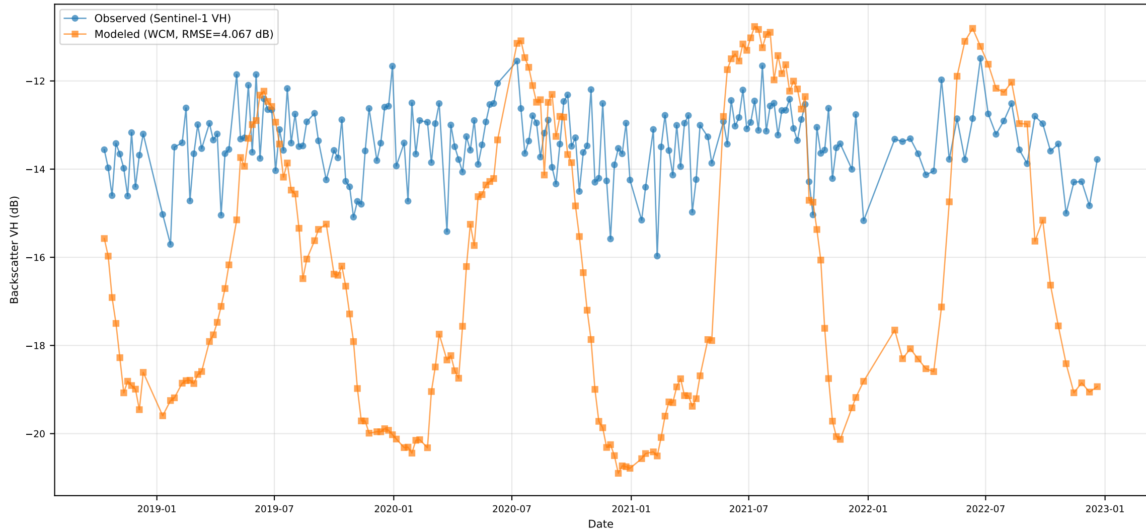
WCM Calibration for VH Polarization Parameters: A=0.018, B=0.09, C=0.01, D=0.001
