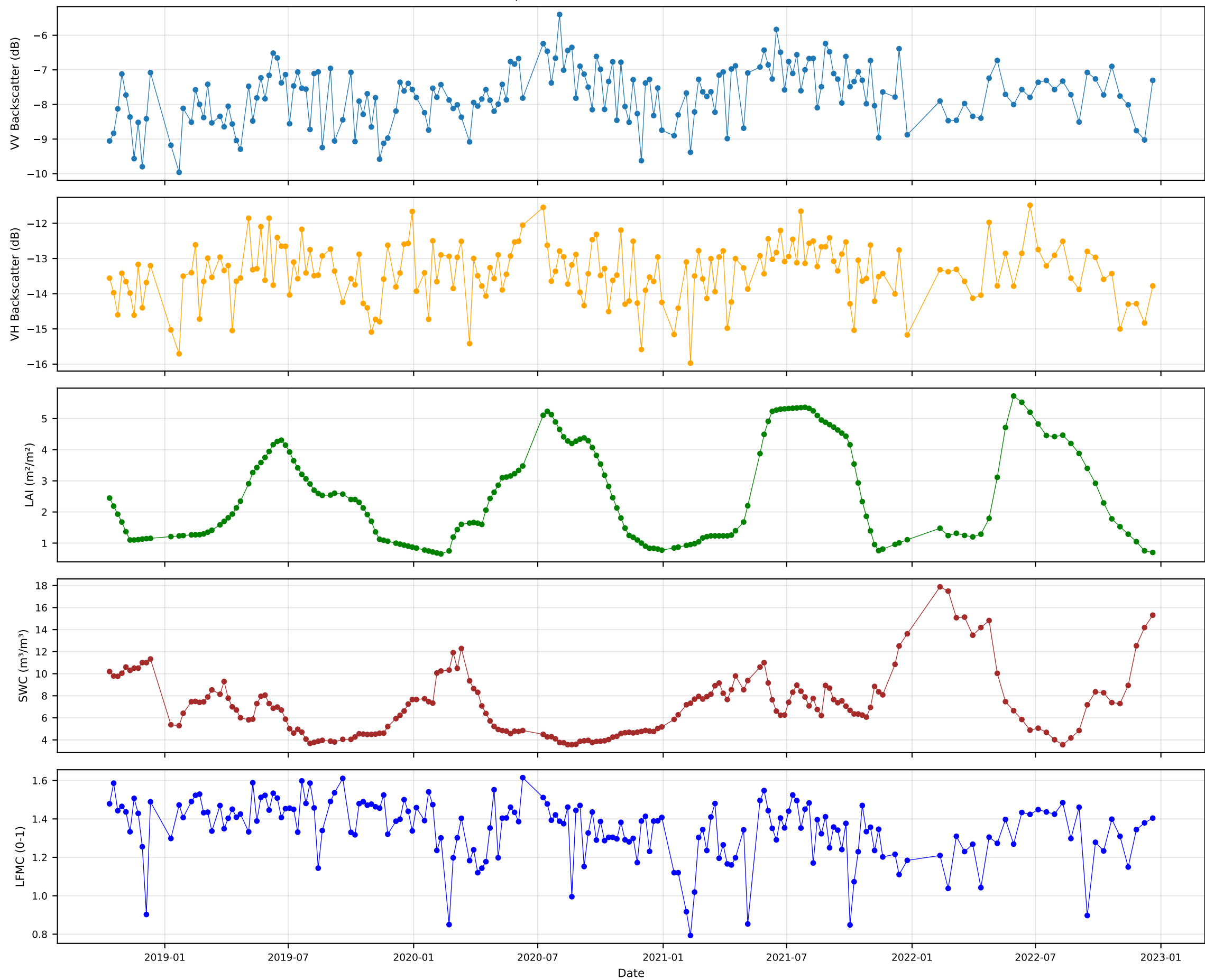
Input Time Series for Water Cloud Model
