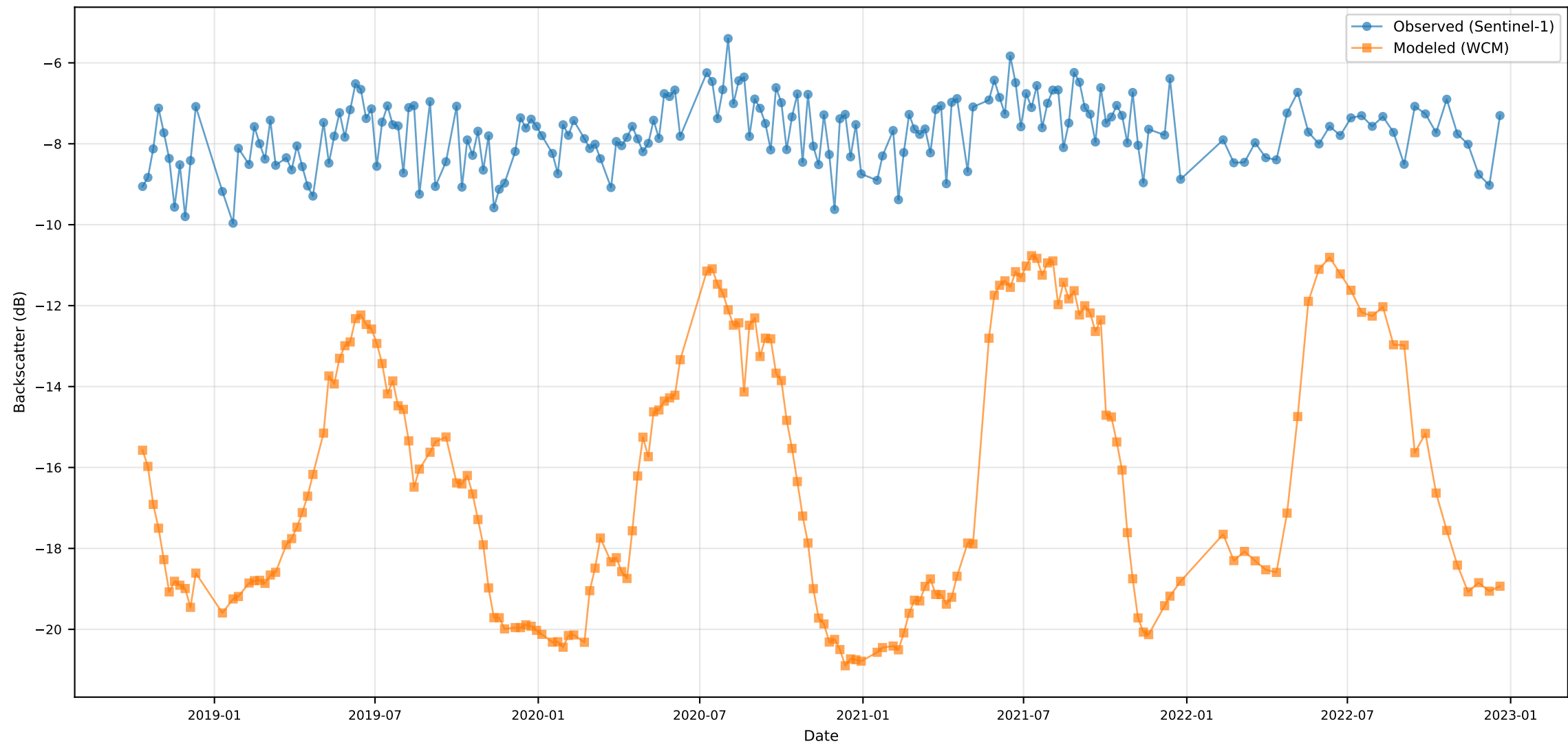
Water Cloud Model vs. Sentinel-1 Observations (VV Polarization)
