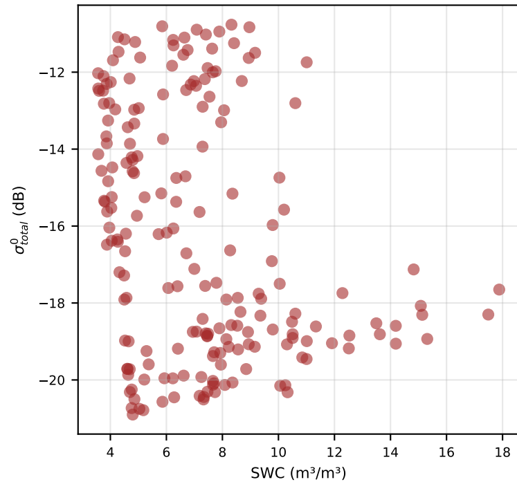
Soil Moisture Influence
