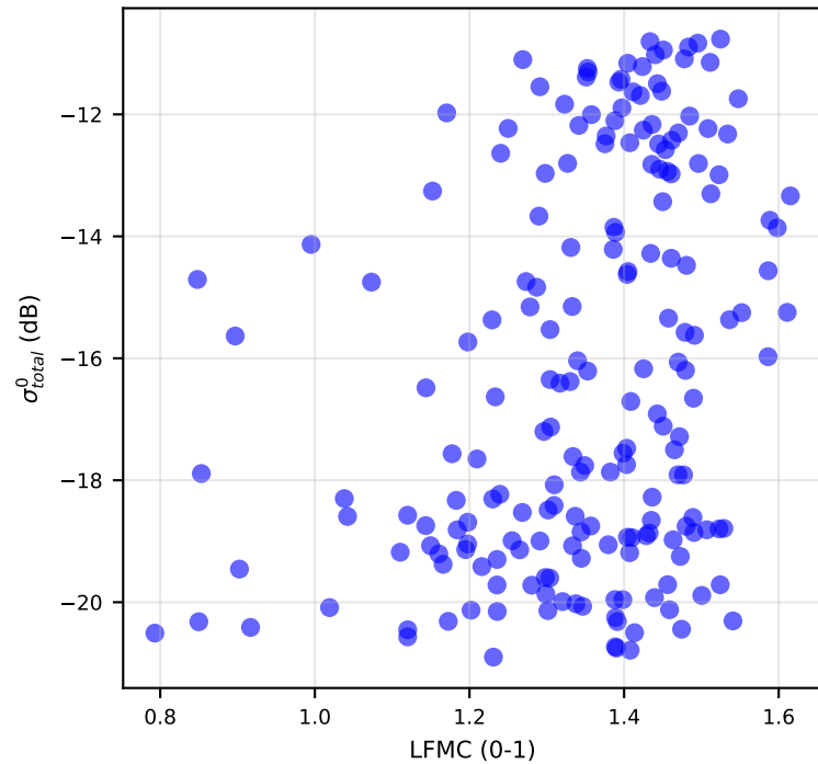
Fuel Moisture Influence
