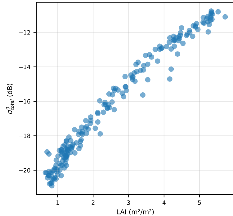
LAI Influence on Backscatter
