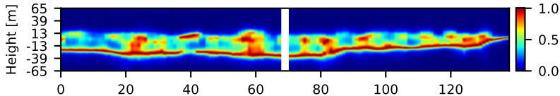
Range slice at azimuth line 108, HH
