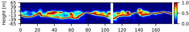
Azimuth slice at range line 69, HH
