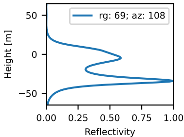
Vertical point profiles, HH
