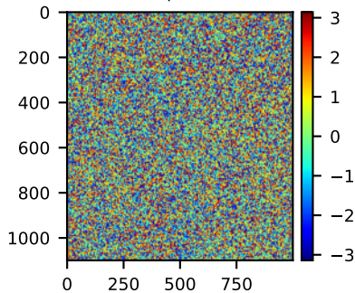
Track 3, phase (rad)
