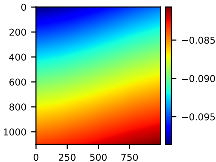
Track 3, vertical wavenumber (rad/m)
