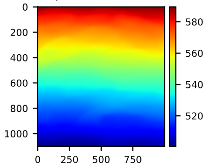
Track 3, phase correction term (rad)
