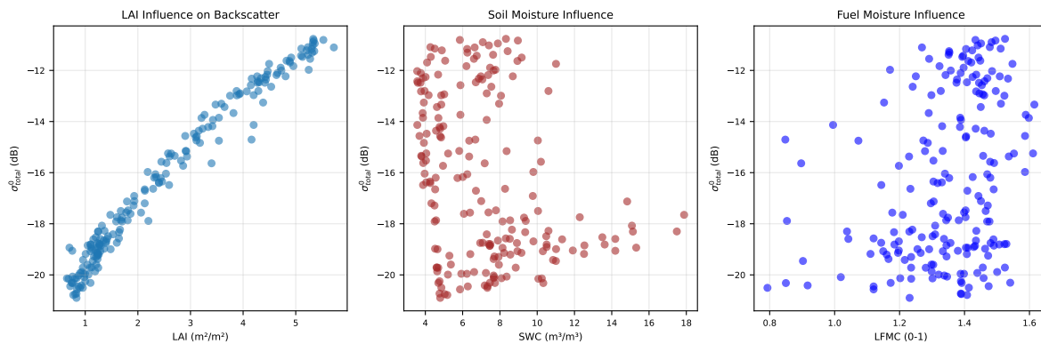
Figure 3: Relationship between modeled backscatter and vegetation parameters
