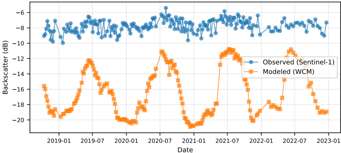
Water Cloud Model vs. Sentinel-1 Observations (VV Polarization)
