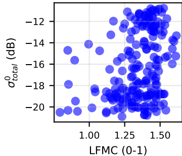
Fuel Moisture Influence
