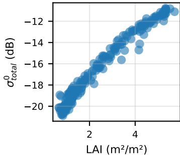
LAI Influence on Backscatter
