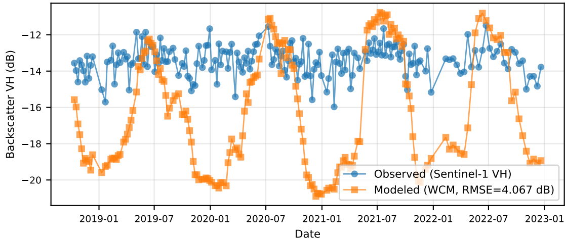
WCM Calibration for VH Polarization Parameters: A=0.018 , B=0.09 , C=0.01 , D=0.001
