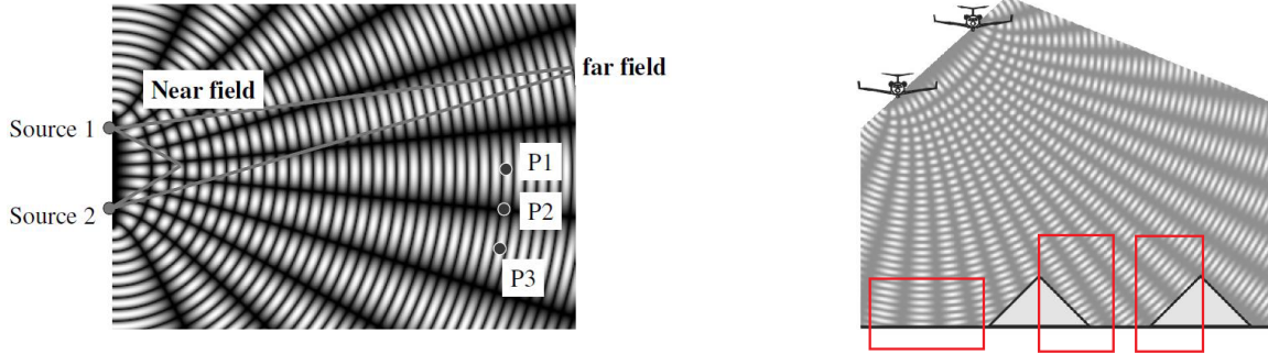
Figure 5: InSAR principle illustrated with interference patterns. Left: Two wave sources create characteristic fringe patterns where waves constructively or destructively interfere. Right: Applying this principle from space, two SAR acquisitions from slightly different positions create interferometric fringes that encode topographic information. Maxima occur when path difference \Delta R = n\lambda , corresponding to phase difference \Delta\phi = n \cdot 2\pi . Source: Iain H. Woodhouse, 2017
