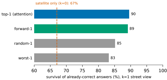
Fig. 5: Survival of already-correct answers when only k=1 street view is kept (Qwen3.6-27B). The forward view (89%) matches attention-selected top-1 (90%) and beats random (85%) and worst (83%); all far exceed the satellite-only floor (67%). Retention over already-correct items, not accuracy.
